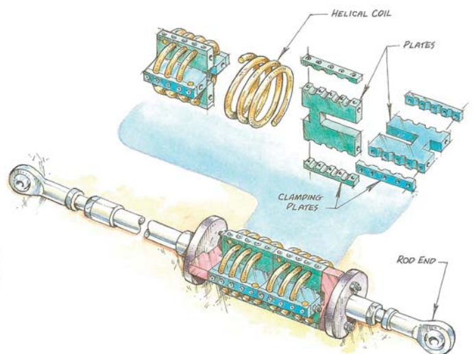
Captured every quarter loop, wire rope coil will not collapse; two-pitch design prevents twisting.
